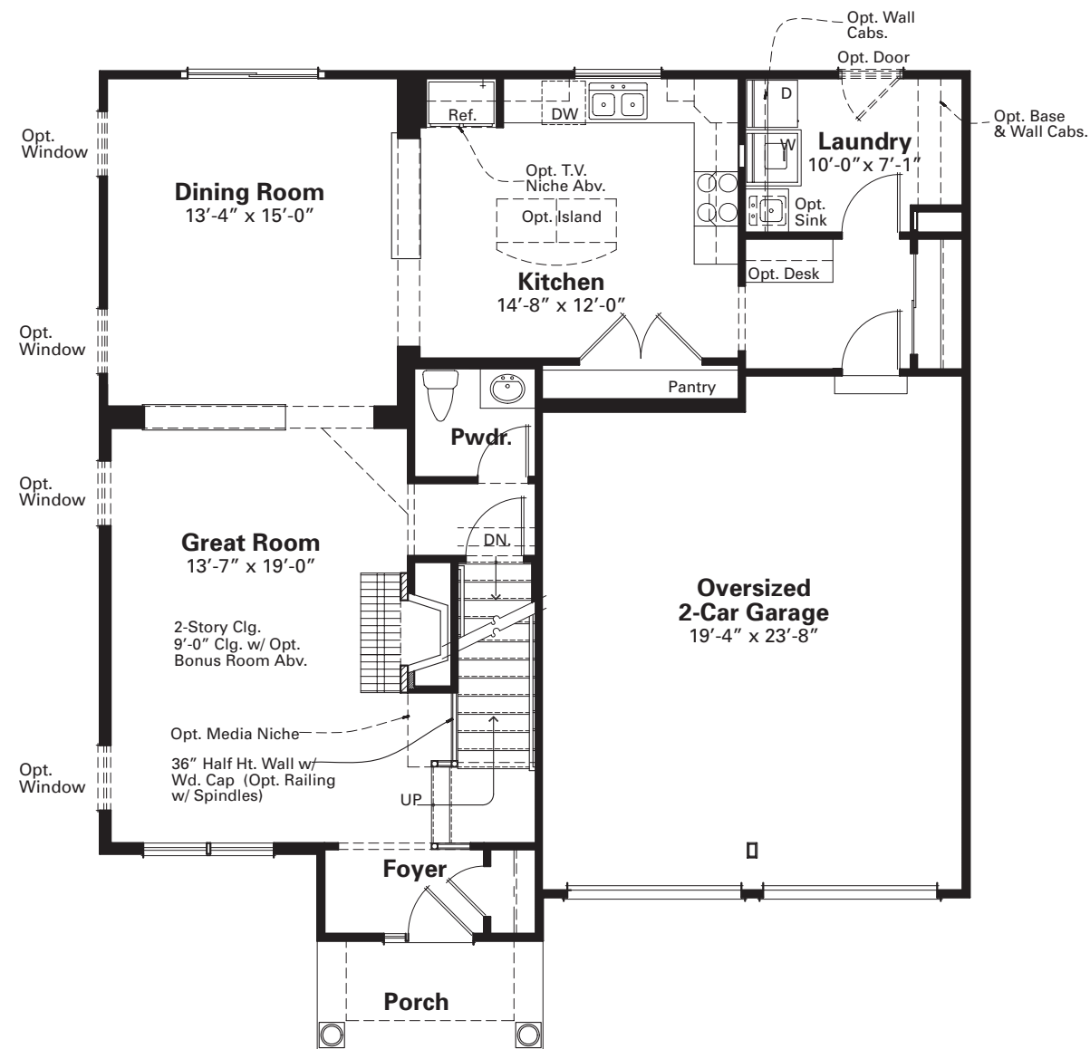
FIRST FLOORPLAN
